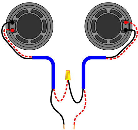
SINGLE WIRED SUBWOOFERS This solution will yield an 8-ohm load. Connect to the outputs of the amplifier.
